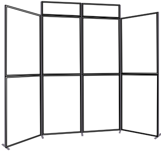
8 panel with 2 optional headers Panels size: 1000mm x 700mm Pole diameter: 16mm
